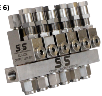
SLS-32 MAG STANDARD VENTING PRESSURE—(US & METRIC CONNECTORS AVAILABLE)
